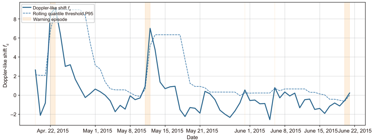
Fig. 2 Cross-scenario validation on the Douban Movie dataset. The release date serves as the retrospective anchor, and shaded regions indicate warning intervals
